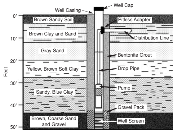
Basic Elements of Well Construction
